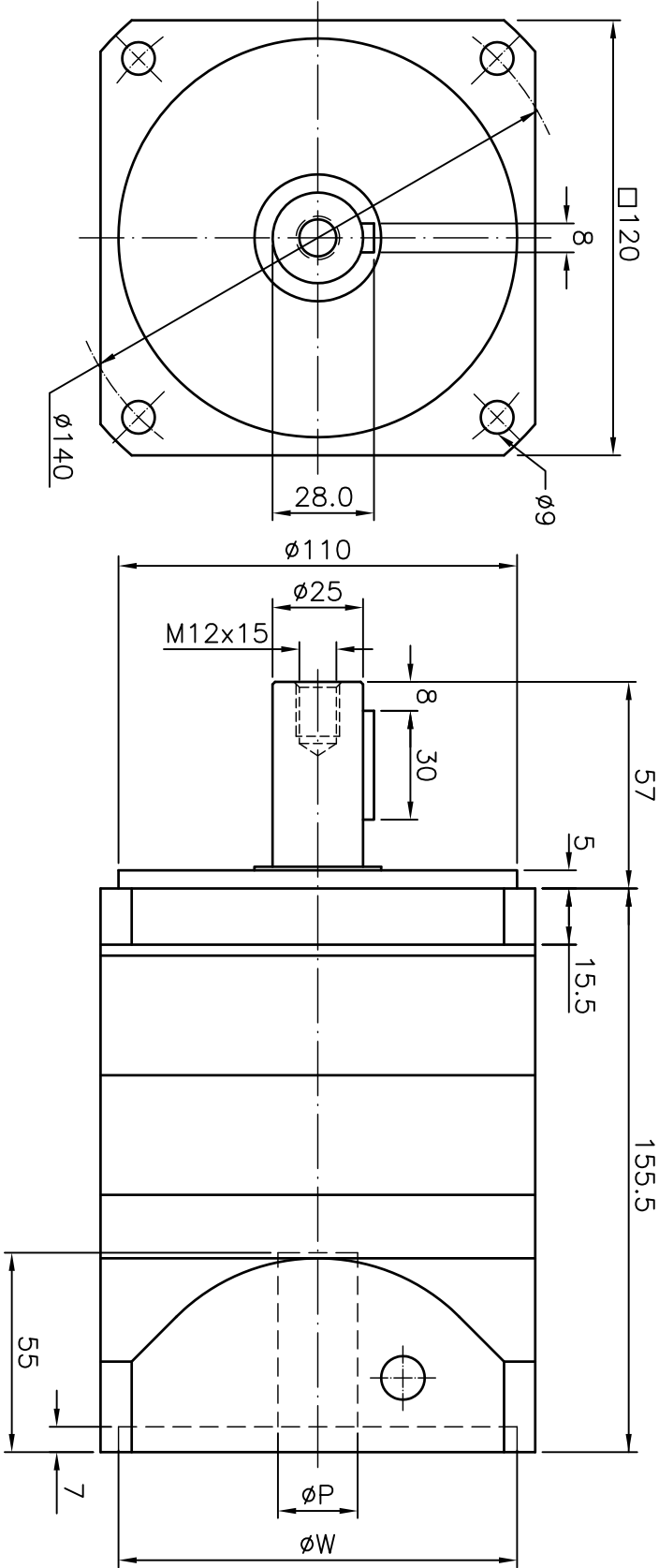
120mm, 2 STAGE, PROFILE DIMENSION
